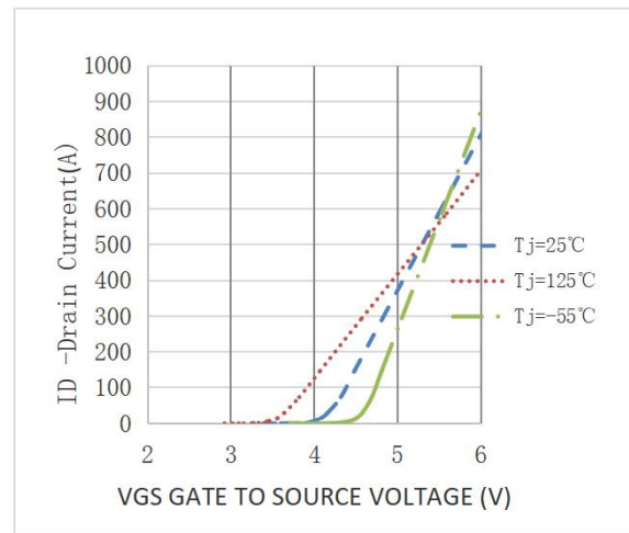
Figure 10. Transfer Characteristics
